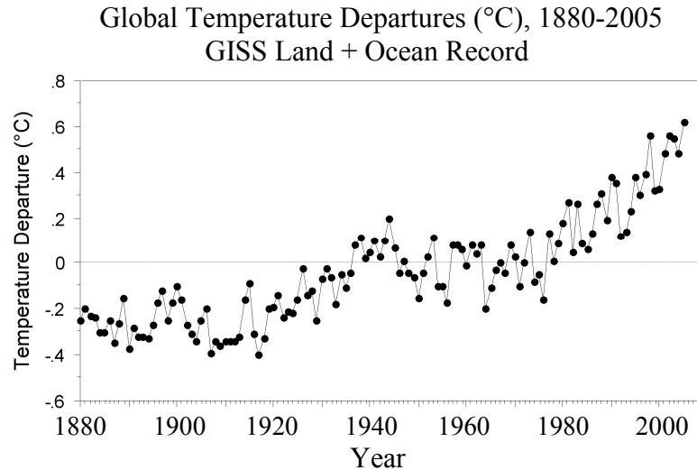
Figure 1. Global Surface Temperature History, NASA Goddard Institute for Space Studies.
